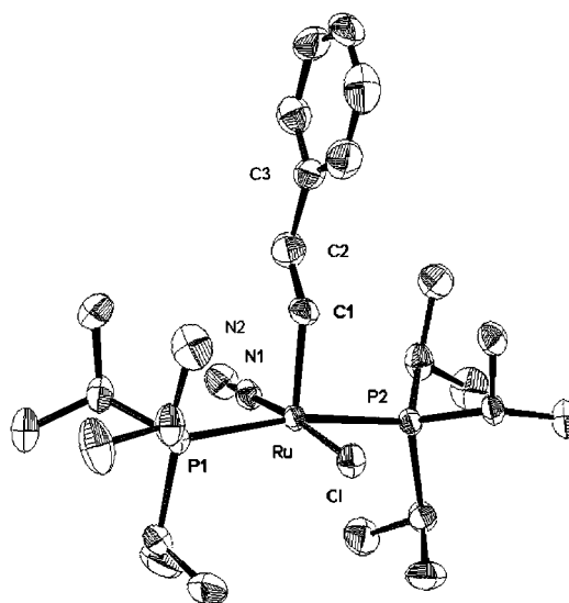
Figure 2. Molecular structure of 29 (hydrogen atoms are omitted for clarity); selected bond lengths [Å] and angles [°]: Ru–P(1) 2.4021(7), Ru–P(2) 2.4005(7), Ru–N(1) 1.869(5), Ru–Cl 2.3959(19), Ru–C(1) 1.973(3), C(1)–C(2) 1.296(5), N(1)–N(2) 1.088(8); P(1)–Ru–P(2) 168.74(3), N(1)–Ru–Cl 174.13(17), P(1)–Ru–Cl 98.15(9), P(2)–Ru–Cl 93.12(9), N(1)–Ru–P(1) 89.42(17), N(1)–Ru–P(2) 90.59(17), Cl–Ru–P(1) 89.33(4), Cl–Ru–P(2) 89.52(4), Cl–Ru–N(1) 90.63(19), Cl–Ru–C(1) 95.23(11), Ru–N(1)–N(2) 179.2(7), Ru–C(1)–C(2) 135.0(3), C(1)–C(2)–C(3) 125.1(3)
