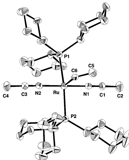
Figure 1. Molecular structure of 26c (hydrogen atoms are omitted for clarity); selected bond lengths [Å] and angles [°]: Ru–P(1) 2.3975(13), Ru–P(2) 2.3979(12), Ru–N(1) 2.008(4), Ru–N(2) 2.006(4), Ru–C(6) 2.001(5), C(6)–C(5) 1.340(7), N(1)–C(1) 1.160(6), N(2)–C(3) 1.142(6); P(1)–Ru–P(2) 171.04(4), N(1)–Ru–N(2) 178.05(15), P(1)–Ru–C(6) 92.48(12), P(2)–Ru–C(6) 96.24(12), N(1)–Ru–C(6) 92.35(16), N(2)–Ru–C(6) 89.52(16), Ru–N(1)–C(1) 176.9(4), Ru–N(2)–C(3) 179.0(4), N(1)–C(1)–C(2) 178.7(5), N(2)–C(3)–C(4) 179.0(5), Ru–C(6)–C(5) 129.8(4)
